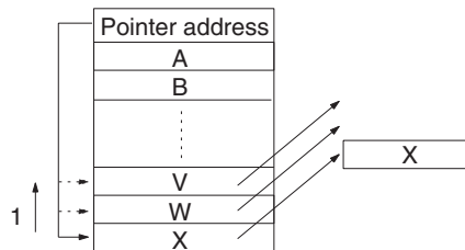
Reads most recent word of data stored in the stack. Each time that a word is read, the pointer is decremented by one to indicate the next address for storage. Data at the position that was read remains unchanged.
